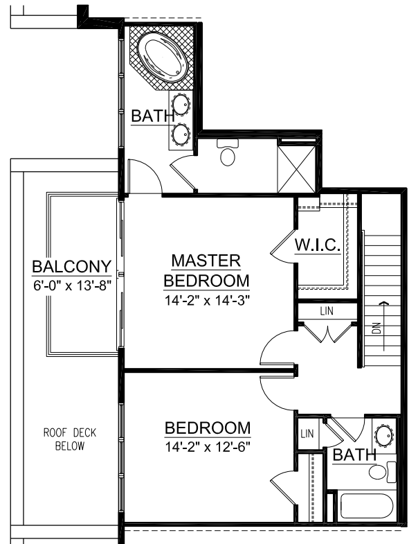
Upper Floor
